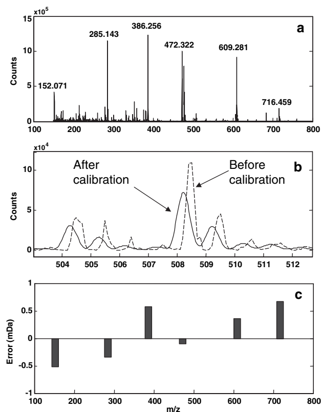
Figure 1. (a) Mass spectrum of the calibration standards. (b) Expanded view of a weak peak before and after calibration. (c) Mass errors for the standard ions used for calibration.
