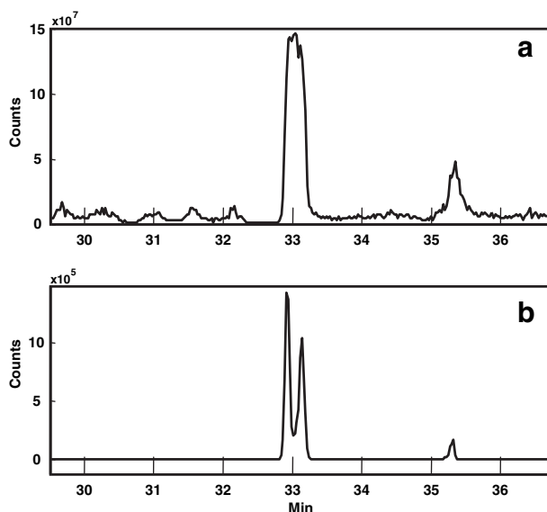
Figure 4. (a) Expanded view of the XIC for m/z 454.8–455.8 Da for the verapamil incubate spiked with a bile matrix. (b) Expanded view of the AMPXIC for the parent drug (verapamil) for the incubate spiked with a bile matrix.
