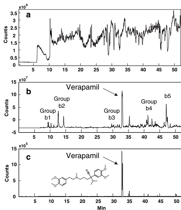
Figure 2. (a) TIC chromatogram for verapamil incubate spiked with a bile matrix. (b) XIC for m/z 454.8–455.8 for verapamil incubate spiked with a bile matrix. (c) AMPXIC for the parent drug (verapamil) for the incubate spiked with a bile matrix.
