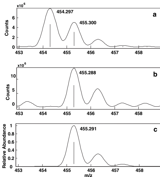
Figure 5. (a) Rejected peak with A+1 ion of MH^+ ion at m/z 455.300 from the verapamil incubate spiked with a bile matrix. (b) Retained peak with monoisotopic m/z 455.288 from the verapamil incubate spiked with a bile matrix. (c) Theoretical mass spectrum of verapamil with monoisotopic MH^+ ion at m/z 455.291.
